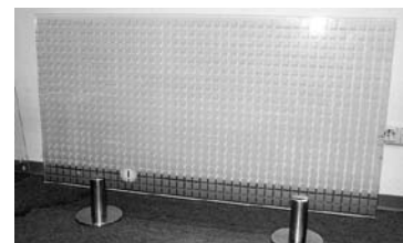
CORRECT !!!
